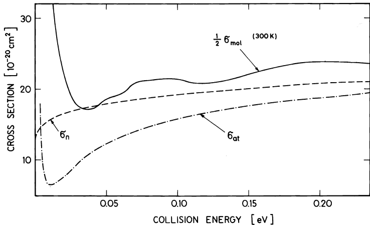
Cross sections for the processes d\mu(\uparrow\downarrow)+d , d\mu(\uparrow\downarrow)+D and d\mu(\uparrow\downarrow)+D_2 averaged over j = 1/2 and j = 3/2 vs collision energy
