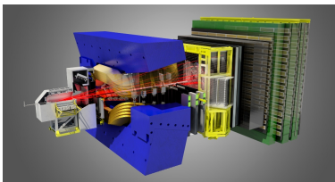
Figure 2.1: The LHCb detector
