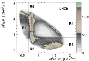
(a) Dalitz plot for \Lambda_c^+ \rightarrow pK^- \pi^+
