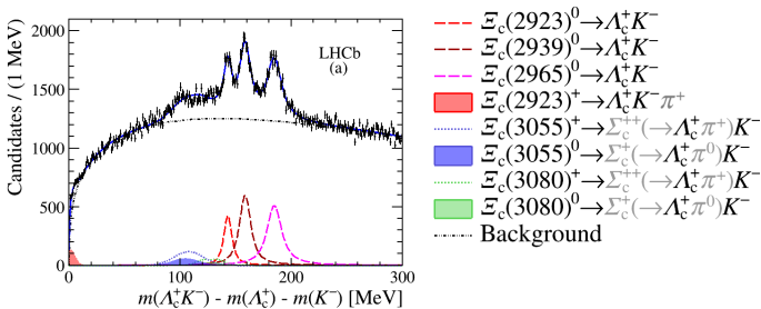
Figure 4.1: Distributions of the invariant-mass difference \Delta M = m(\Lambda_c^+ K^-) - m(\Lambda_c^+) - m(K^-)
