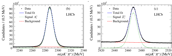
Figure 5.3: Distributions of the mass spectrum M(pK^- \pi^+) Left: \Lambda_c^+ region, Right: \Xi_c^+ region
