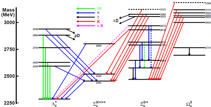
Figure 1.1: Charmed baryon spectrum as in Ref. [2] (provided by Heavy Flavor Averaging Group).
