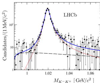
Figure 3.2: Left: Fit results for the \Xi_c^+ \rightarrow pK^-K^+ decay ( \phi region: M_{K^-K^+} < 1.07\text{GeV}/c^2 ) Right: Background subtracted K^-K^+ mass distribution for the \Xi_c^+ \rightarrow pK^-K^+ decay
