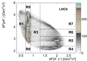
(b) Dalitz plot for \Xi_c^+ \rightarrow pK^- \pi^+
