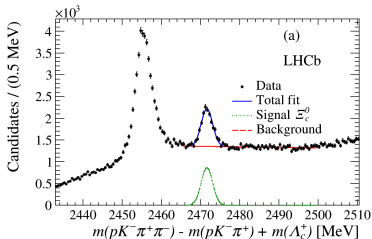
Figure 5.2: Reconstructed invariant-mass distribution and signal fit of M(pK^- \pi^+ \pi^-)
